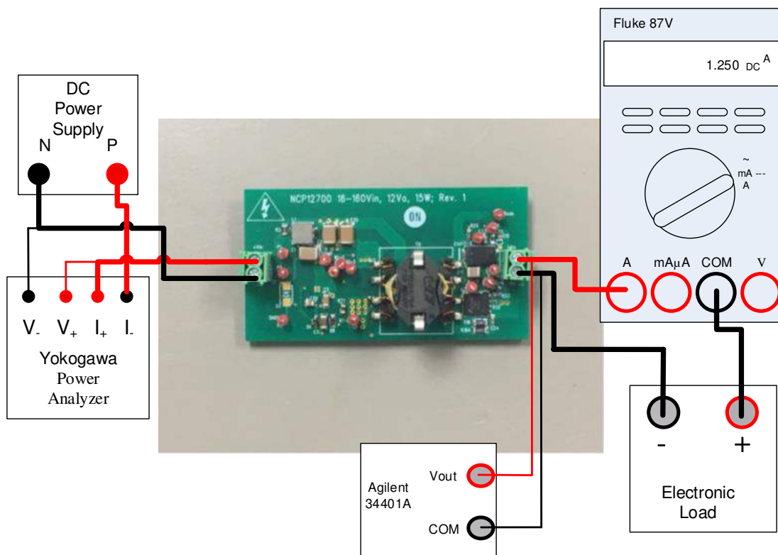
Figure 1: Test Setup
