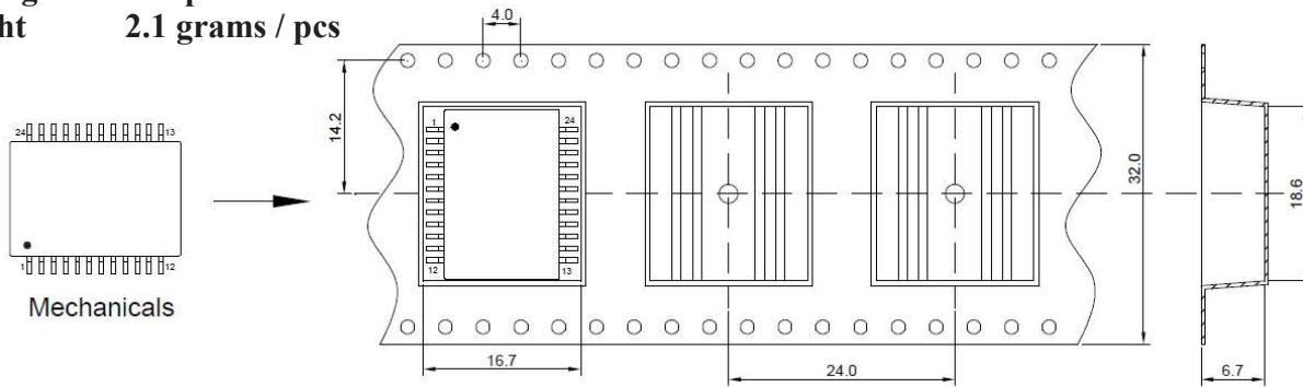
Tape & Reel
