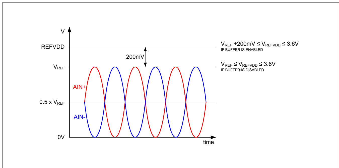
Figure 1. Signal Ranges
