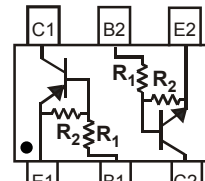
R1, R2 Device Schematic
