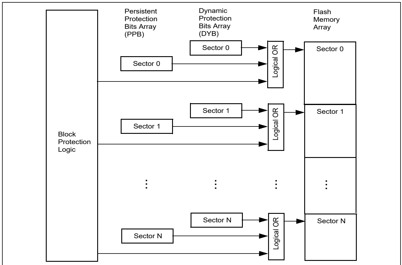
Figure 39 Sector protection control
