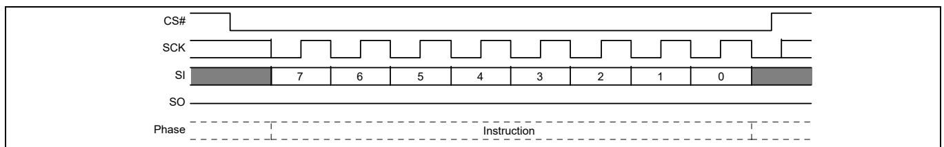
Figure 102 Mode Bit Reset command sequence
