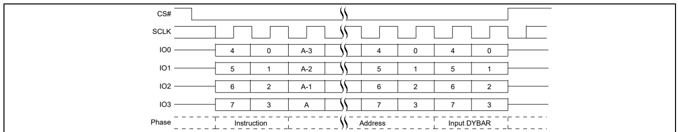
Figure 92 DYBWR QPI mode command sequence [59, 60]
