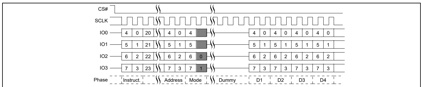
Figure 67 Quad I/O Read command sequence (3-byte address, EBh [CR2V[7] = 0]) QPI mode
