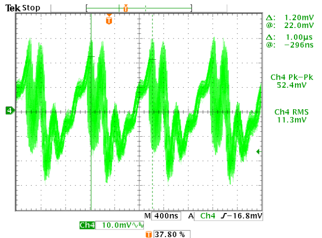
Figure 40. Input Voltage Noise, No Interleave
