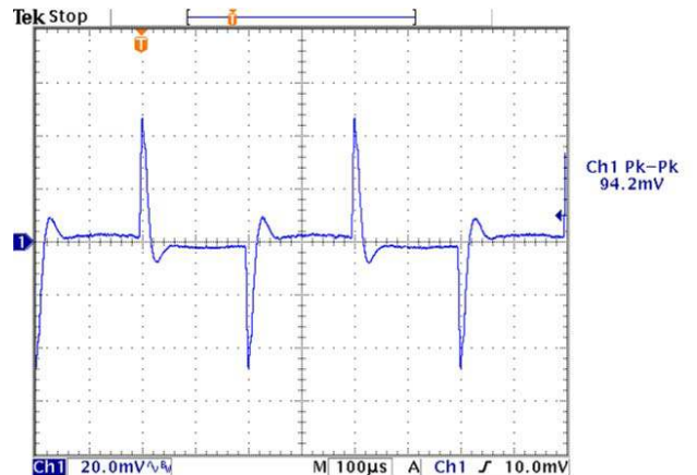
Figure 21. Transient Response without Optimal Voltage Positioning
