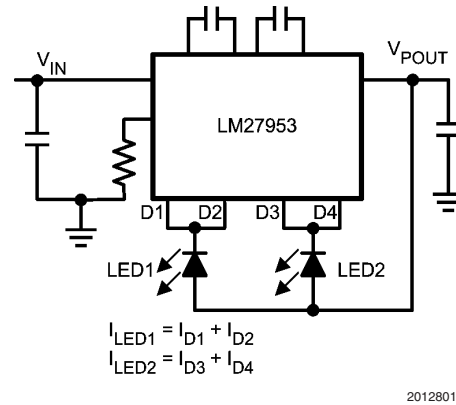
FIGURE 1. Two Parallel Connected LEDs
