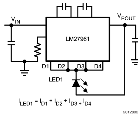
FIGURE 2. One Parallel Connected LED
