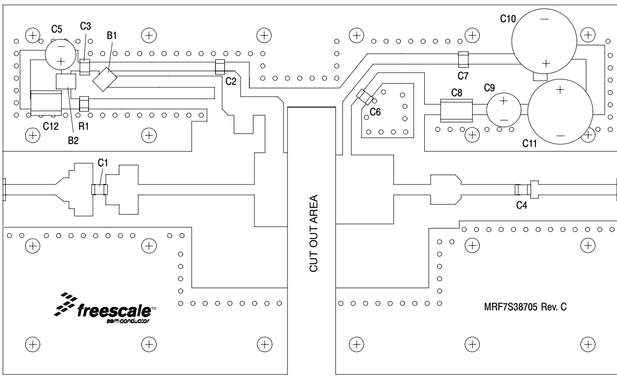
Figure 2. MRF7S38075HR3(HSR3) Test Circuit Component Layout
