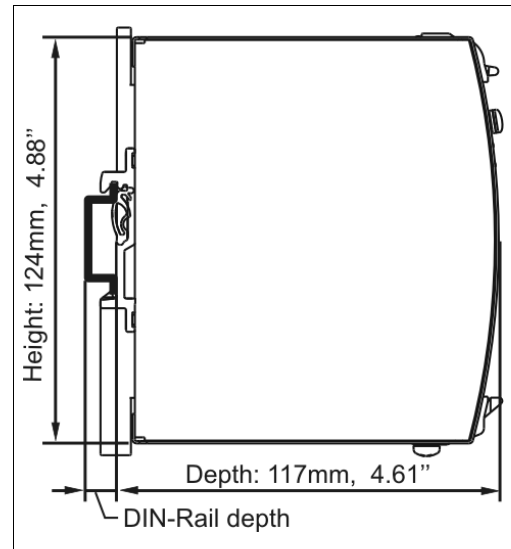
Fig. 22-2 Side view
