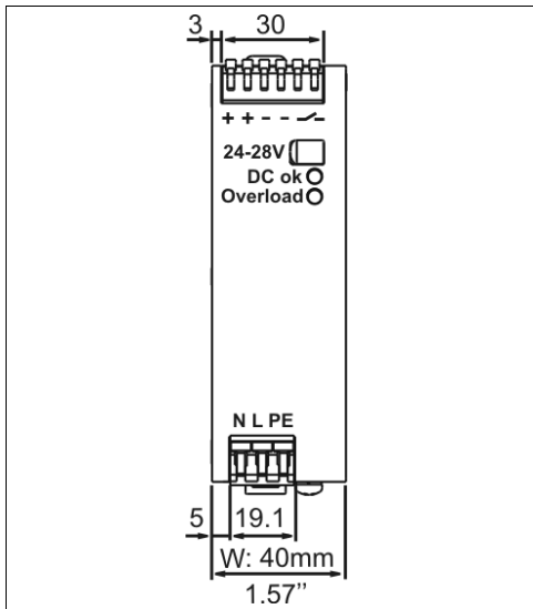
Fig. 22-1 Front view
