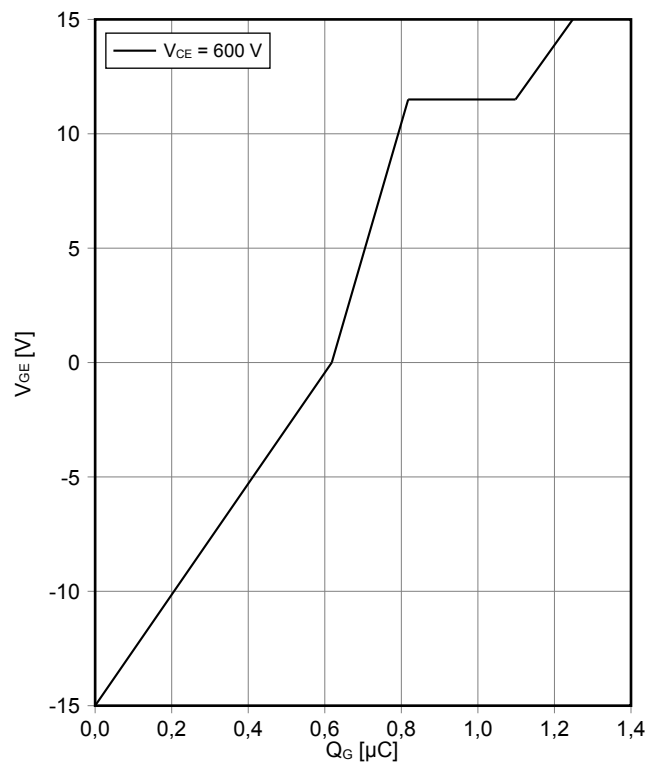
Gateladungs Charakteristik IGBT, Wechselrichter (typisch) gate charge characteristic IGBT, Inverter (typical) V_{GE} = f(Q_G) I_C = 75\text{ A} , T_{vj} = 25^\circ\text{C}
