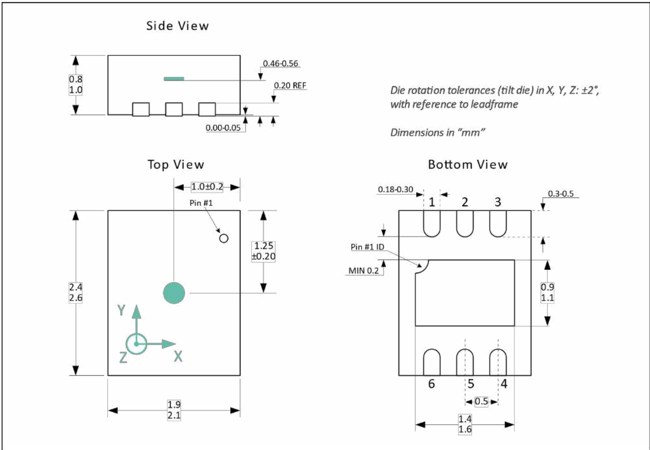
Figure 20 – DFN-6 package dimensions and sensitive spot location
