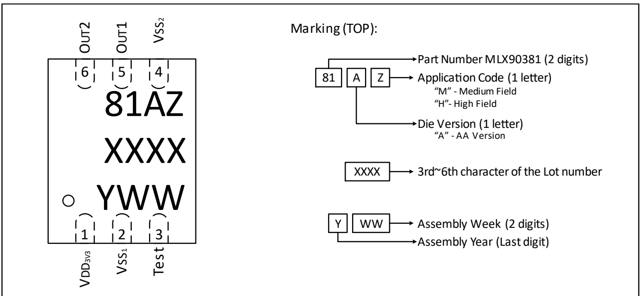
Figure 21 – DFN-6 pin out and marking
