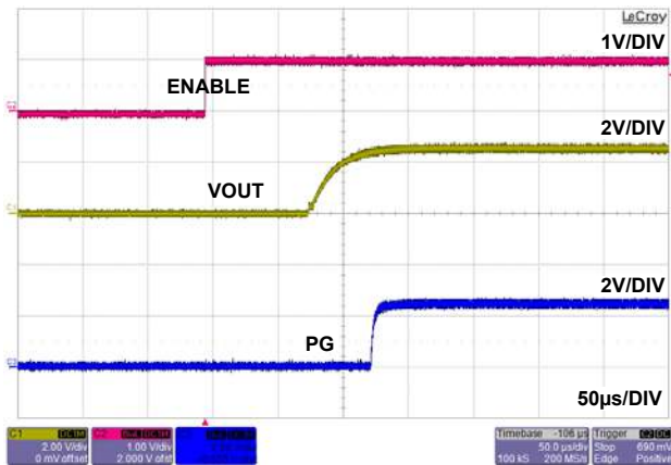
FIGURE 7. START-UP WAVEFORMS
