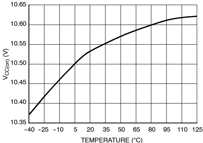
Figure 17. V CC(on)
