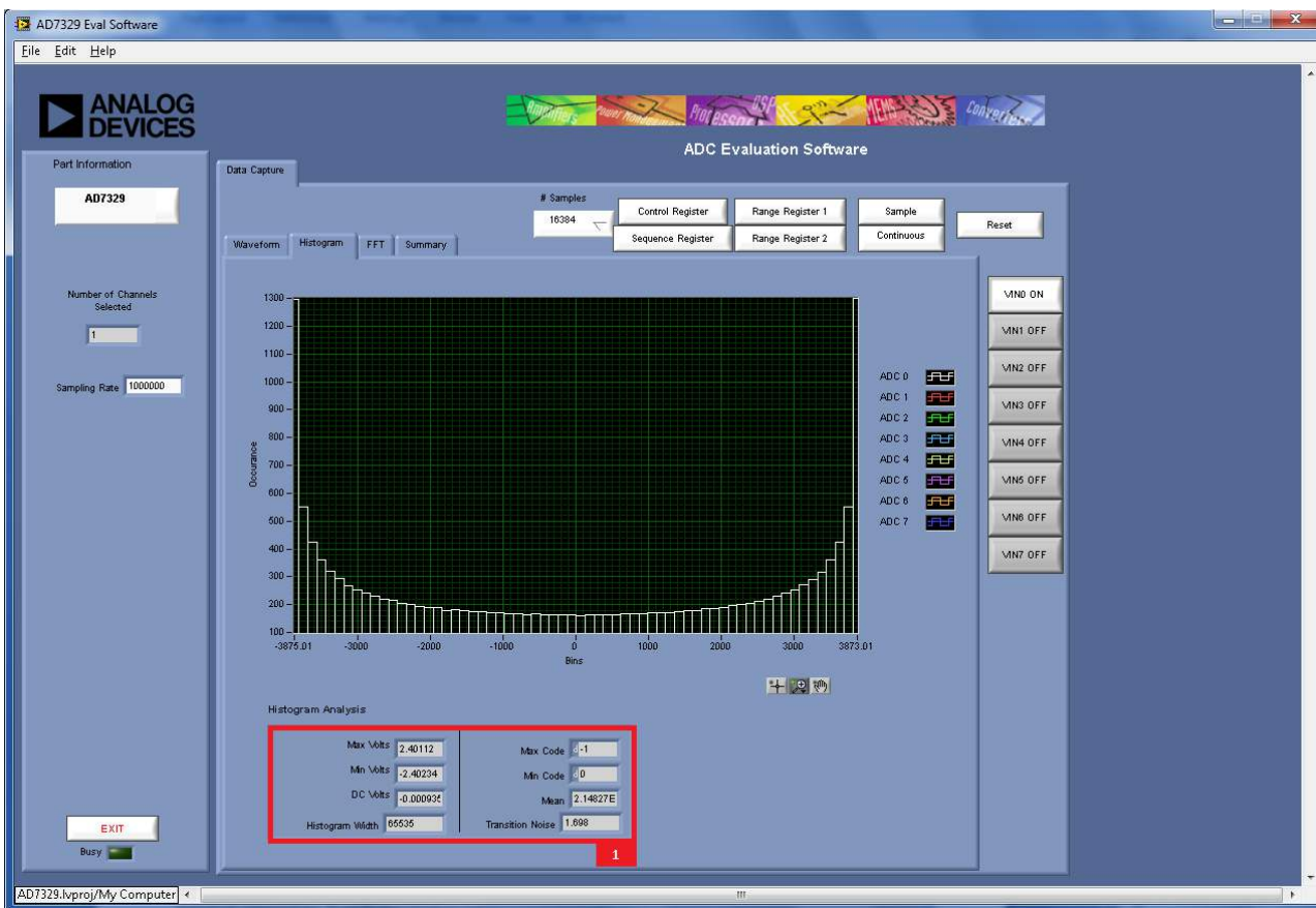
Figure 23. Histogram Tab
