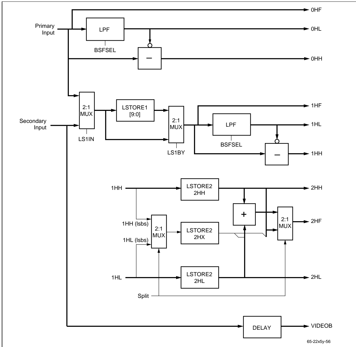
Figure 15. Block Diagram of Comb Filter Input
