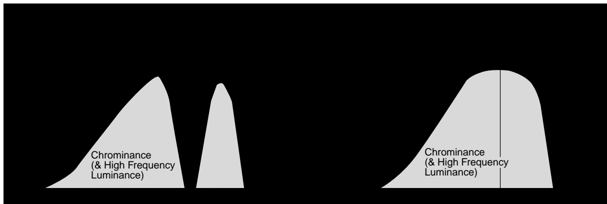
Figure 5. Examples of Notch and Bandpass Filters
