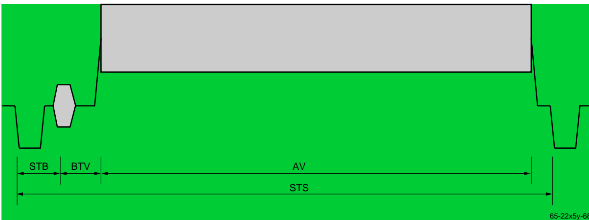
Figure 27. Horizontal Timing
