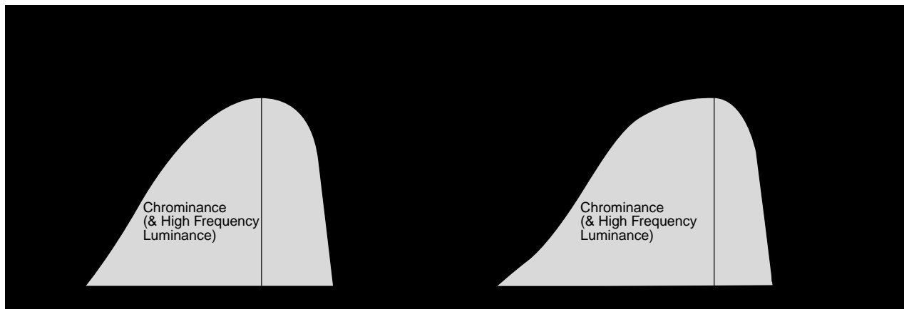
Figure 4. Comparison of the Frequency Spectrum of NTSC and PAL Composite Video Signals
