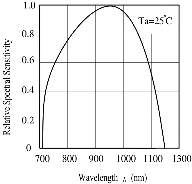
Fig.1 Spectral Sensitivity
