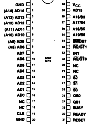
Figure 2. 8087 Pin Configuration
