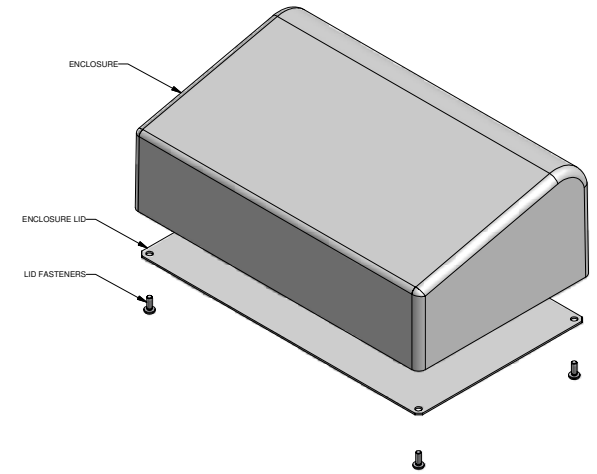
ENCLOSURE ASSEMBLY
