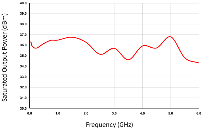
Figure 3. Saturated Output Power Performance (P SAT ) vs Frequency
