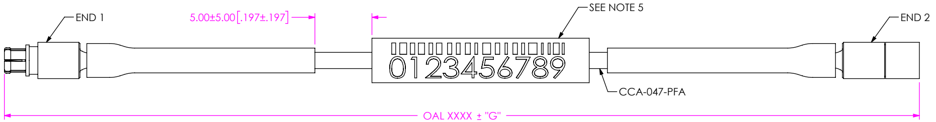
FIG 1 RF047-A-M0SJ-M0SP-XXXX SHOWN (PROTECTIVE CAPS NOT SHOWN FOR CLARITY)
