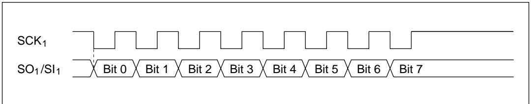
Figure 10-2 Transfer Format
