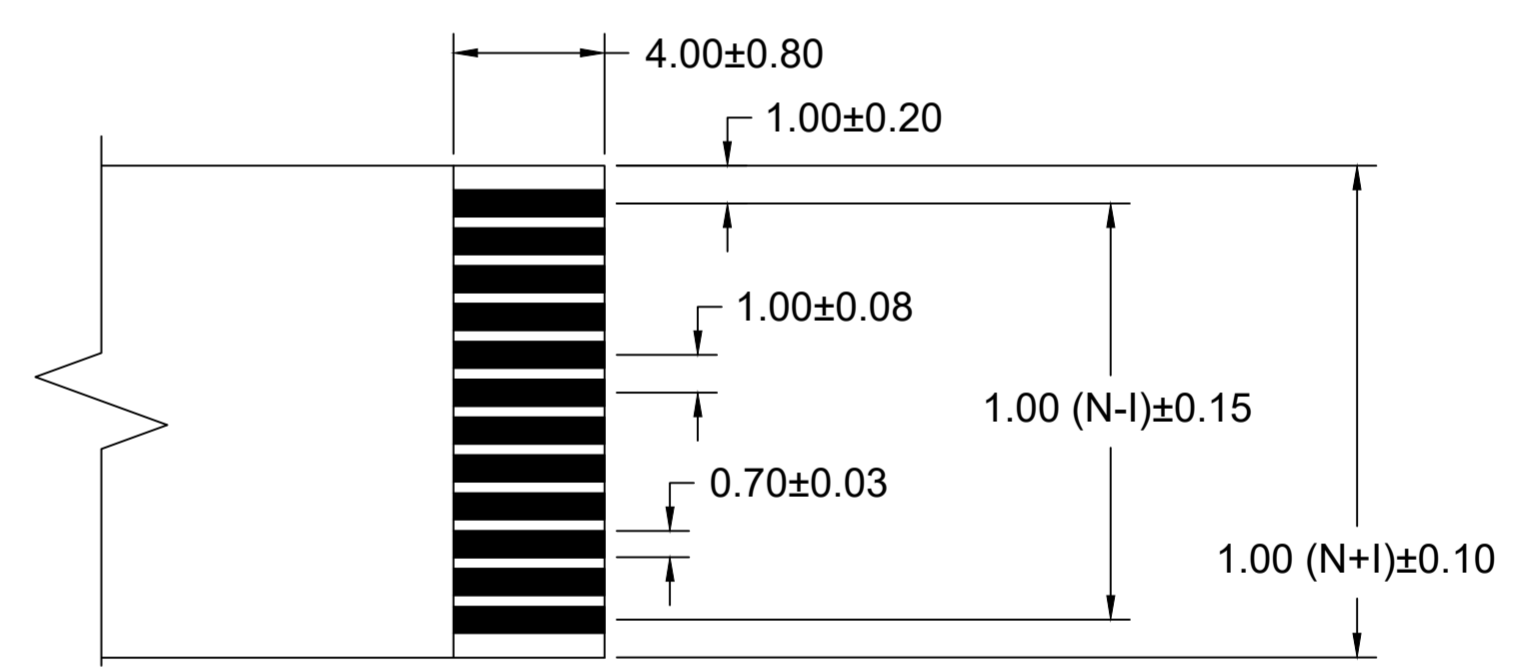
END TAIL DETAIL SCALE 5:1
