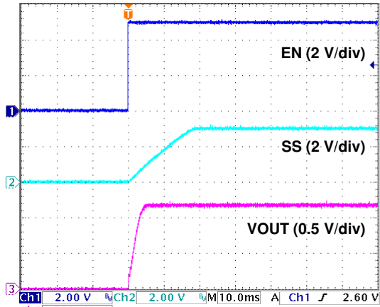
Time (10 ms/div)
