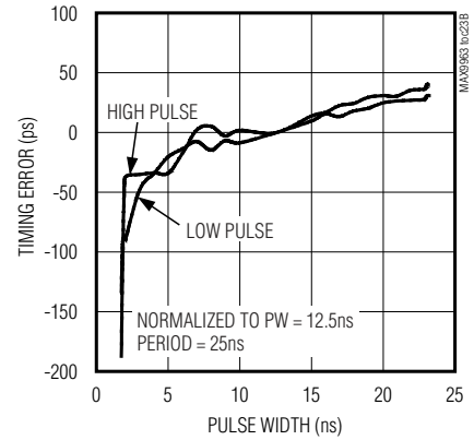
COMPARATOR TRAILING-EDGE TIMING ERROR vs. PULSE WIDTH, MAX9963_JCCQ
