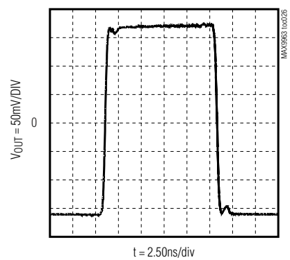
COMPARATOR DIFFERENTIAL OUTPUT RESPONSE, MAX9963_GCCQ
