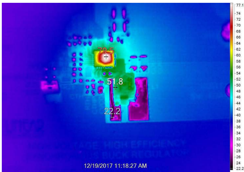
Figure 4. Thermal Map, V_{IN} 14V, I_{OUT} 1 5V at 4A, No Air Flow
