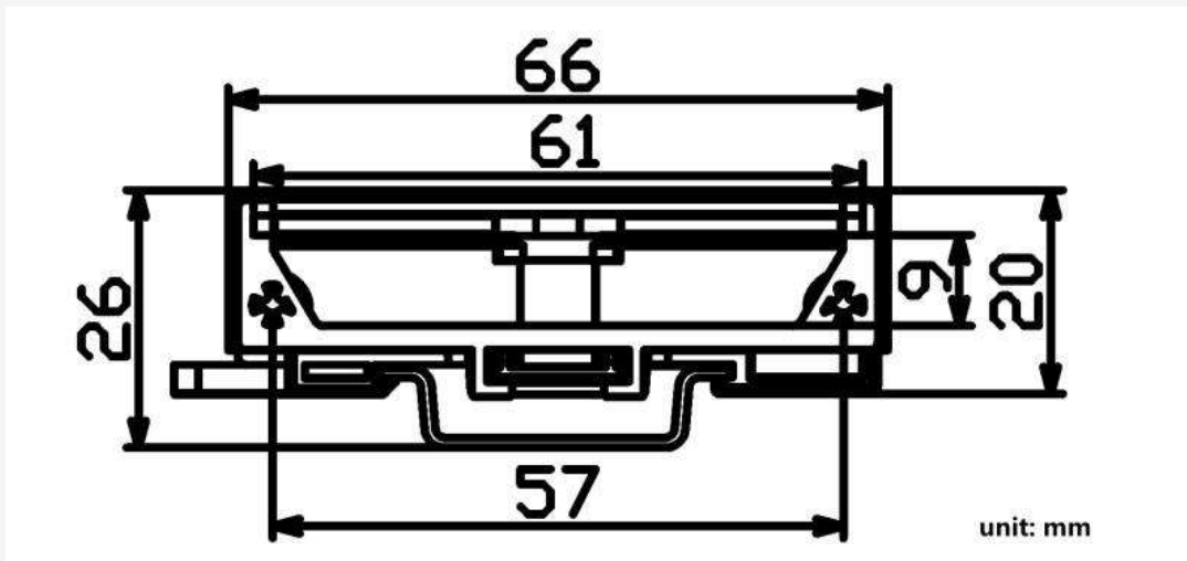
Dimension of Rail Mount Bracket
