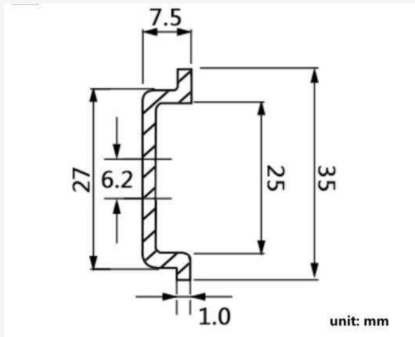
Dimension of Rail Mount Adapter
