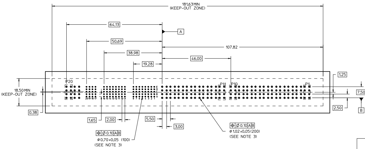
RECOMMENDED PCB LAYOUT AND KEEP-OUT ZONE
