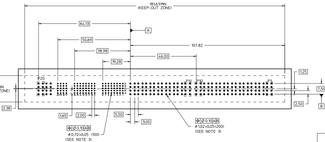
RECOMMENDED PCB LAYOUT AND KEEP-OUT ZONE
