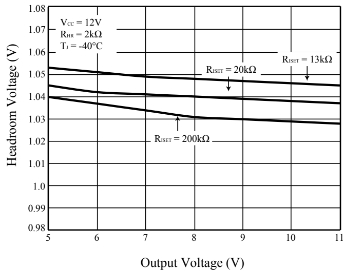
Figure 13 V_{HR} vs. V_{OUT}
