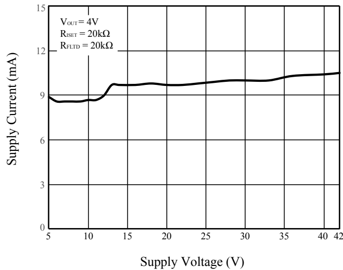
Figure 17 I_{CC} vs. V_{CC}
