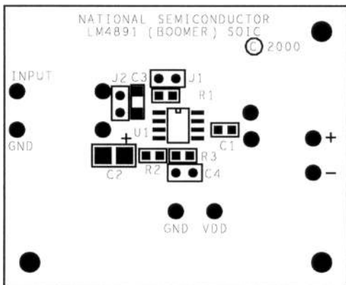
Figure 40. Silk Screen
