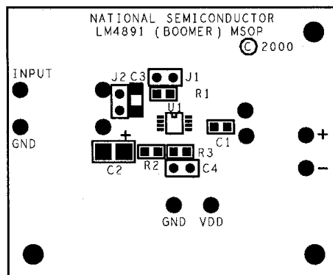
Figure 43. Silk Screen
