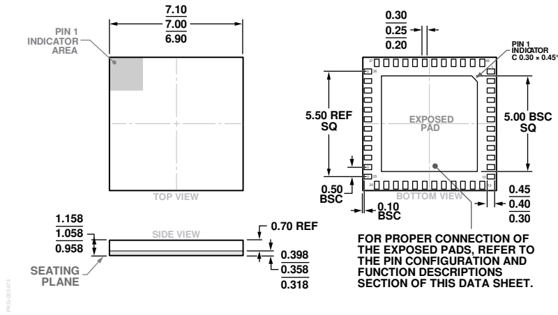
Figure 38. 48-Terminal Land Grid Array [LGA] (CC-48-4) Dimensions shown in millimeters
