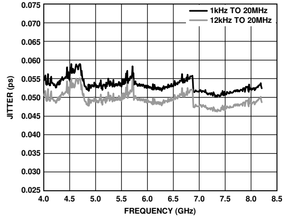
Figure 22. RMS Jitter, Fractional-N, f_{PFD} = 153.6 \text{ MHz} , V_{CC\_VCO} = 5 \text{ V}
