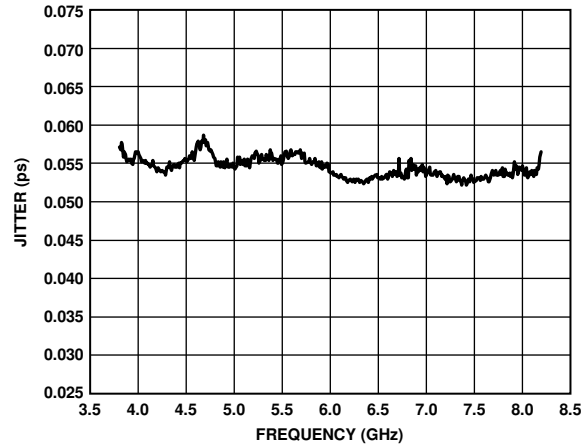
Figure 23. RMS Jitter Integrated from 1 kHz to 100 MHz, Fractional-N, f_{PFD} = 153.6 \text{ MHz} , V_{CC\_VCO} = 3.3 \text{ V}
