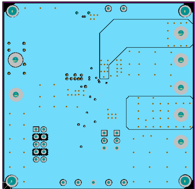
Figure 4—Middle Layer2
