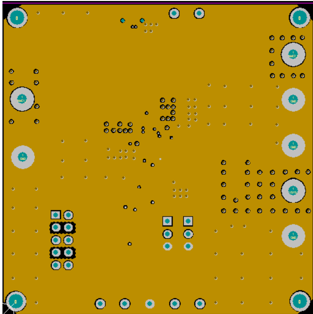
Figure 3—Middle Layer1
