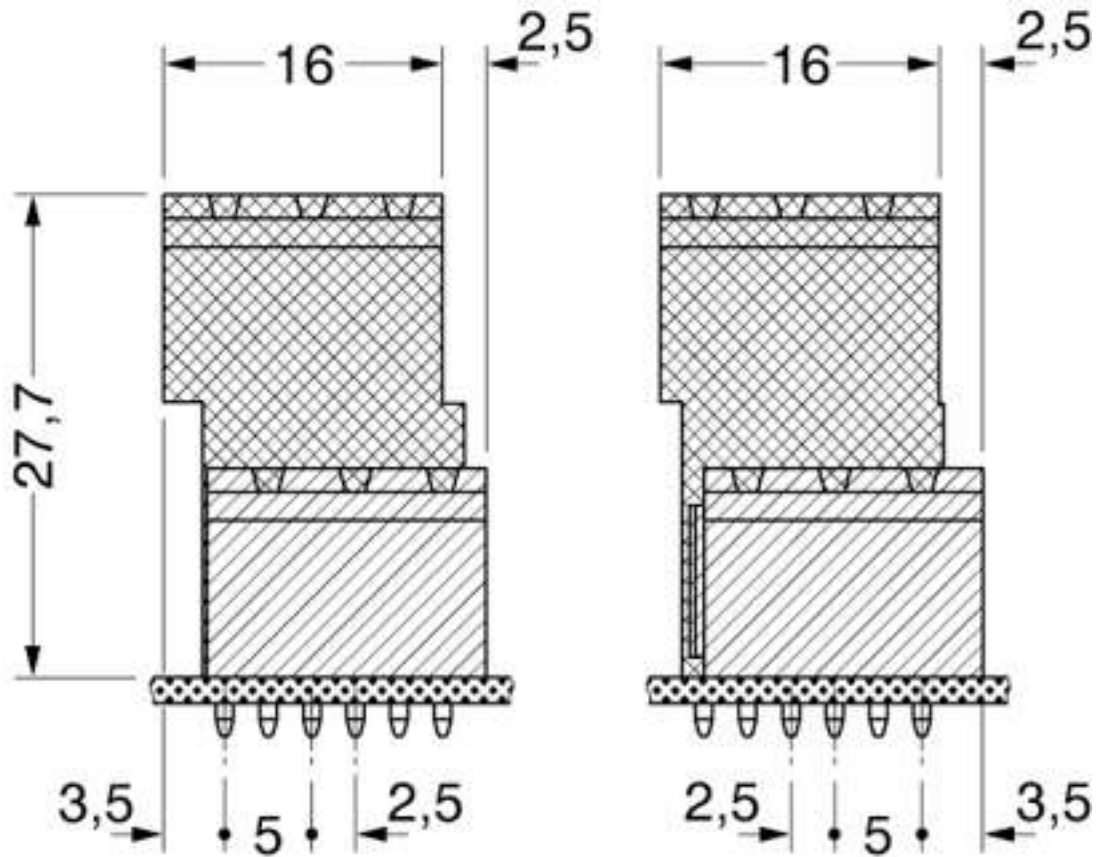
Dimensioned drawing
