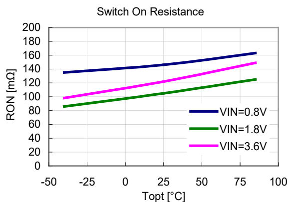
15) Switch on resistance vs. Temperature
