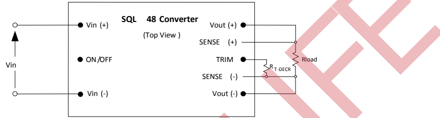
Figure D. Configuration for decreasing output voltage.
