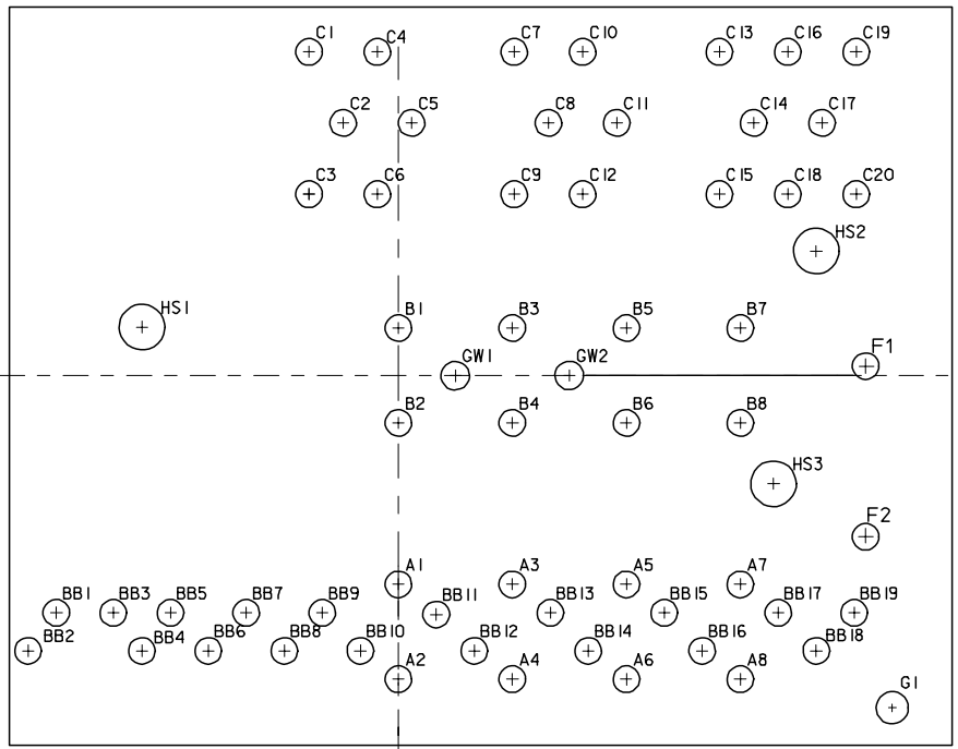
RECOMMENDED REAR P.C.B. LAYOUT THICKNESS 1.6 ±0.20
