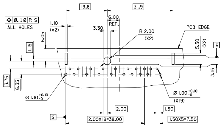
RECOMMENDED MAIN P.C.B. LAYOUT THICKNESS 1.6 ±0.20 SCALE 2:1
