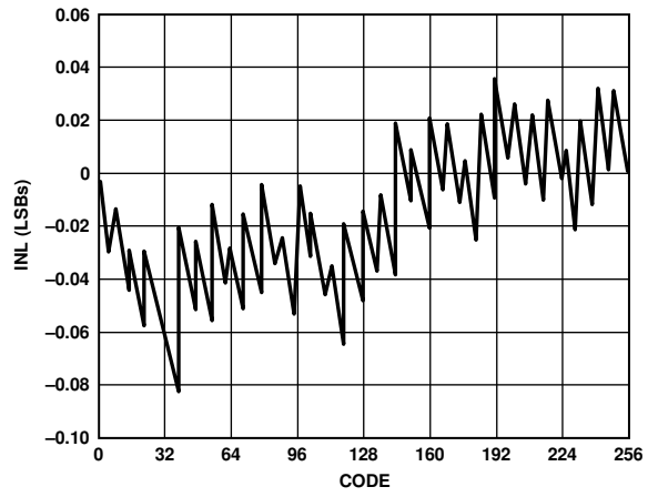
Figure 14. Typical INL
