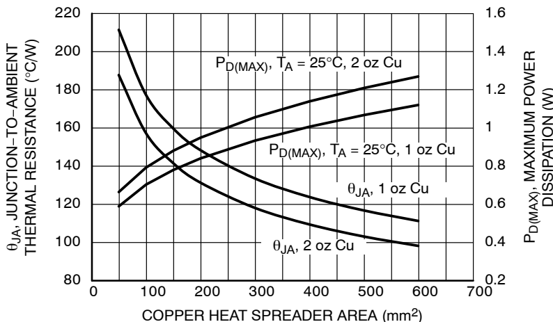
Figure 66. θ JA and P D(MAX) vs. Copper Area (WDFN6)
