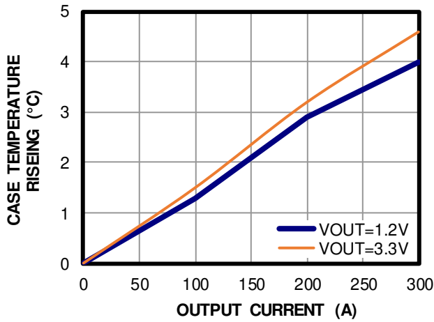
Case Temp Rising vs. Output Current
