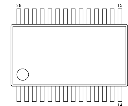
28-Lead Small Outline Integrated Circuit (SOIC), MS-013, 0.300" Wide Body Package Number M28B
