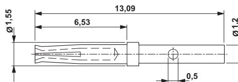
Dimensioned drawing
