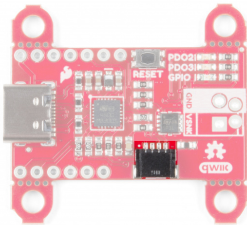
Qwiic Connector
