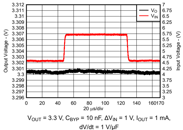
Figure 8-18. Line Transient Response for New Chip
