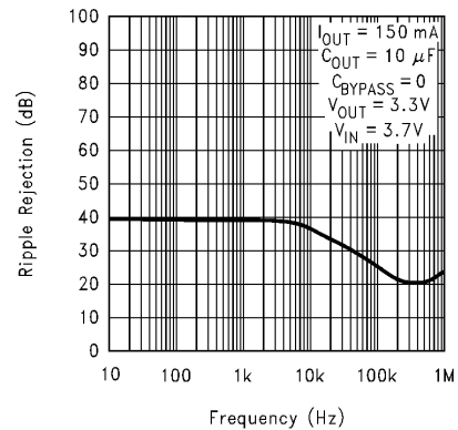
Figure 6-10. Ripple Rejection vs Frequency for Legacy Chip
