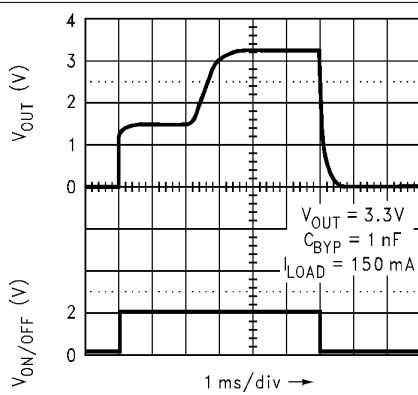
Figure 8-25. Turn-On Time for Legacy Chip
