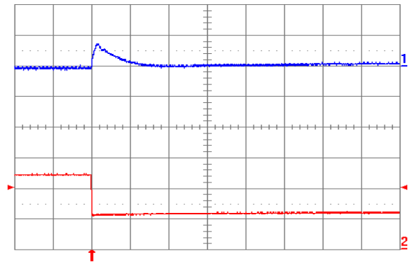
Fig. 2.5V.8: Output voltage response for V_{out} = 2.5\text{ V} to negative load current step change from 5 A to 2.5 A with slew rate of -5 A/ \mu\text{s} at V_{in} = 12\text{ V} . Top trace: output voltage (100 mV/div.); Bottom trace: load current (2 A/div.). C_o = 100\text{ }\mu\text{F} ceramic. Time scale: 20 \mu\text{s} /div.
