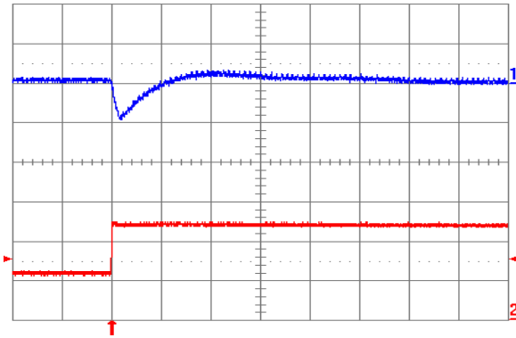
Fig. 3.3V.7: Output voltage response for V_{out} = 3.3\text{ V} to positive load current step change from 2.5 A to 5 A with slew rate of 5\text{ A}/\mu\text{s} at V_{in} = 12\text{ V} . Top trace: output voltage (100 mV/div.); Bottom trace: load current (2 A/div.). C_o = 100\ \mu\text{F} ceramic. Time scale: 20 \mu\text{s} /div.
