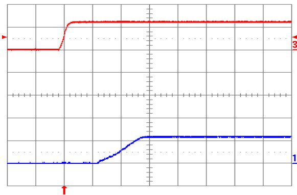
Fig. 1.2V.5: Turn-on transient for V_{out} = 1.2\text{ V} with application of V_{in} at full rated load current (resistive) and 100\text{ }\mu\text{F} external capacitance at V_{in} = 12\text{ V} . Top trace: V_{in} (10 V/div.); Bottom trace: output voltage (1 V/div.); Time scale: 5 ms/div.
