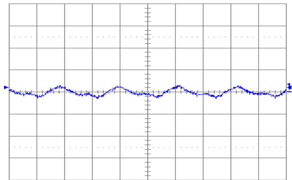
Fig. 5.0V.6: Output voltage ripple (20 mV/div.) at full rated load current into a resistive load with external capacitance 100 \mu\text{F} ceramic and V_{in} = 12\text{ V} for V_{out} = 5.0\text{ V} . Time scale: 1 \mu\text{s} /div.
