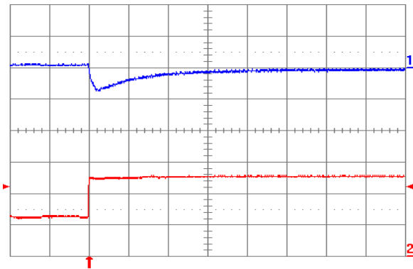
Fig. 1.0V.7: Output voltage response for V_{out} = 1.0\text{ V} to positive load current step change from 2.5\text{ A} to 5\text{ A} with slew rate of 5\text{ A}/\mu\text{s} at V_{in} = 12\text{ V} . Top trace: output voltage ( 100\text{ mV/div.} ); Bottom trace: load current ( 2\text{ A/div.} ). C_o = 100\ \mu\text{F} ceramic. Time scale: 20\ \mu\text{s/div.}
