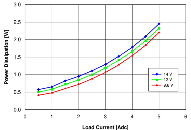
Fig. 2.0V.4: Power Loss vs. load current and input voltage for V_{out} = 2.0\text{ V} converter mounted vertically with air flowing at a rate of 200 LFM (1 m/s) and T_a = 25\text{ }^\circ\text{C}
