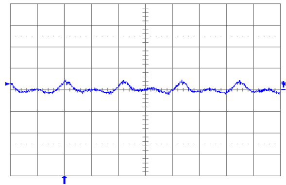
Fig. 2.5V.6: Output voltage ripple (20 mV/div.) at full rated load current into a resistive load with external capacitance 100 \mu\text{F} ceramic + 1 \mu\text{F} ceramic and V_{in} = 12\text{ V} for V_{out} = 2.5\text{ V} . Time scale: 2 \mu\text{s} /div.
