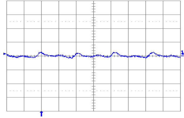
Fig. 1.0V.6: Output voltage ripple ( 20\text{ mV/div.} ) at full rated load current into a resistive load with external capacitance 100\ \mu\text{F} ceramic and V_{in} = 12\text{ V} for V_{out} = 1.0\text{ V} . Time scale: 1\ \mu\text{s/div.}
