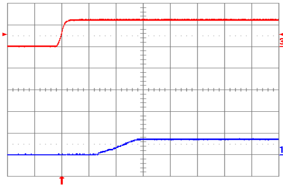
Fig. 0.7525V.5: Turn-on transient for V_{out} = 0.7525\text{ V} with application of V_{in} at full rated load current (resistive) and 100\text{ }\mu\text{F} external capacitance at V_{in} = 12\text{ V} . Top trace: V_{in} (10 V/div.); Bottom trace: output voltage (1 V/div.); Time scale: 5 ms/div.
