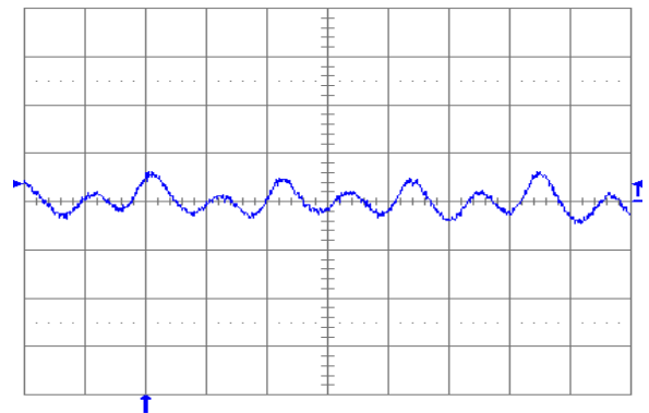
Fig. 2.0V.6: Output voltage ripple (20 mV/div.) at full rated load current into a resistive load with external capacitance 100 \mu\text{F} ceramic and V_{in} = 12\text{ V} for V_{out} = 2.0\text{ V} . Time scale: 1 \mu\text{s} /div.
