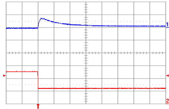
Fig. 1.0V.8: Output voltage response for V_{out} = 1.0\text{ V} to negative load current step change from 5\text{ A} to 2.5\text{ A} with slew rate of -5\text{ A}/\mu\text{s} at V_{in} = 12\text{ V} . Top trace: output voltage ( 100\text{ mV/div.} ); Bottom trace: load current ( 2\text{ A/div.} ). C_o = 100\ \mu\text{F} ceramic. Time scale: 20\ \mu\text{s/div.}
