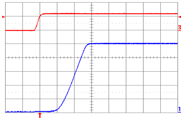
Fig. 5.0V.5: Turn-on transient for V_{out} = 5.0\text{ V} with application of V_{in} at full rated load current (resistive) and 100 \mu\text{F} external capacitance at V_{in} = 12\text{ V} . Top trace: V_{in} (10 V/div.); Bottom trace: output voltage (1 V/div.); Time scale: 5 ms/div.
