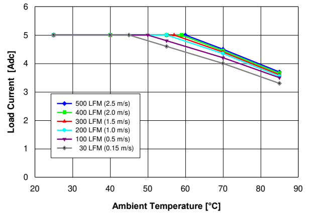
Fig. 2.0V.2: Available load current vs. ambient temperature and airflow rates for V_{out} = 2.0\text{ V} converter mounted horizontally with V_{in} = 12\text{ V} , and maximum MOSFET temperature \leq 120\text{ }^\circ\text{C} .
