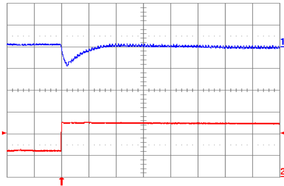
Fig. 2.5V.7: Output voltage response for V_{out} = 2.5\text{ V} to positive load current step change from 2.5 A to 5 A with slew rate of 5 A/ \mu\text{s} at V_{in} = 12\text{ V} . Top trace: output voltage (100 mV/div.); Bottom trace: load current (2 A/div.). C_o = 100\text{ }\mu\text{F} ceramic. Time scale: 20 \mu\text{s} /div.
