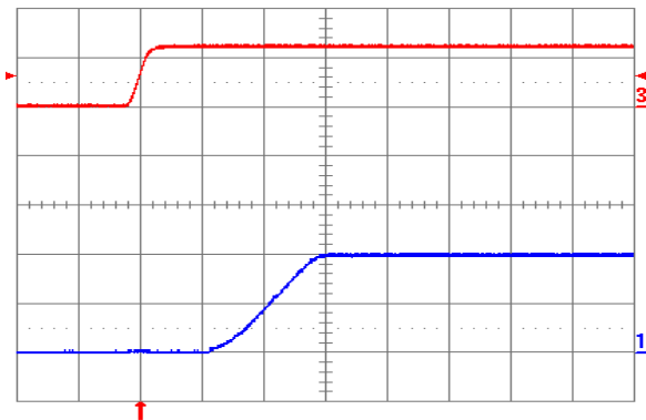
Fig. 2.0V.5: Turn-on transient for V_{out} = 2.0\text{ V} with application of V_{in} at full rated load current (resistive) and 100 \mu\text{F} external capacitance at V_{in} = 12\text{ V} . Top trace: V_{in} (10 V/div.); Bottom trace: output voltage (1 V/div.); Time scale: 5 ms/div.
