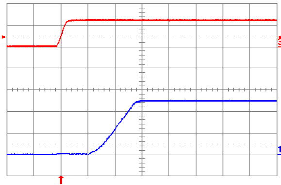
Fig. 2.5V.5: Turn-on transient for V_{out} = 2.5\text{ V} with application of V_{in} at full rated load current (resistive) and 100 \mu\text{F} external capacitance at V_{in} = 12\text{ V} . Top trace: V_{in} (10 V/div.); Bottom trace: output voltage (1 V/div.); Time scale: 5 ms/div.
