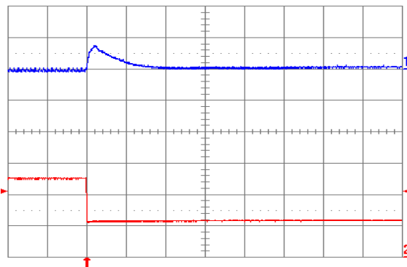
Fig. 2.0V.8: Output voltage response for V_{out} = 2.0\text{ V} to negative load current step change from 5 A to 2.5 A with slew rate of -5\text{ A}/\mu\text{s} at V_{in} = 12\text{ V} . Top trace: output voltage (100 mV/div.); Bottom trace: load current (2 A/div.). C_o = 100\text{ }\mu\text{F} ceramic. Time scale: 20\text{ }\mu\text{s}/\text{div} .
