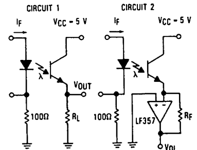
Switching Time Test Circuit
