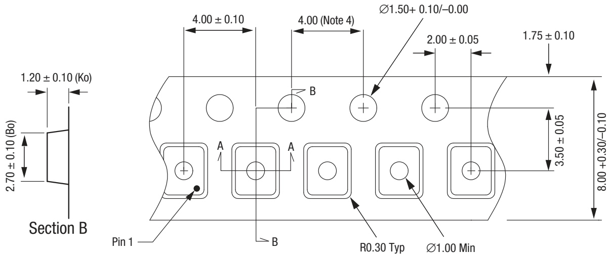
Figure 9. SC-88 Package Dimension Drawing
