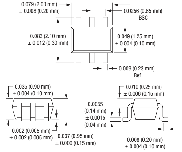
Dimensions are in inches (millimeters shown in parentheses) 200043-009
