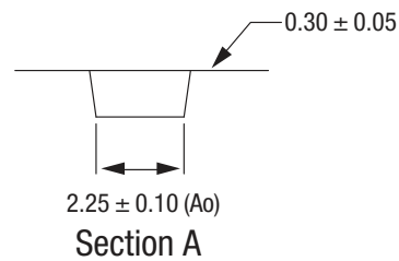
Figure 10. SC-88 Tape and Reel Dimensions
