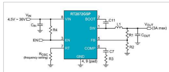
36V/3A buck converter for automotive applications.
