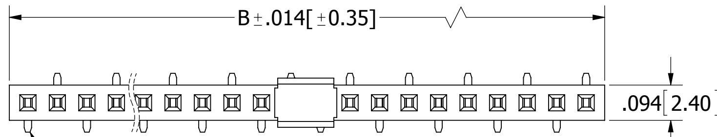
xPxNxx1BFLD-M81RC (OPPOSITE BEND, APPLICABLE ON EVEN COUNTS)
