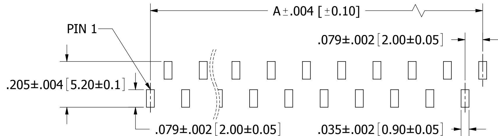
RECOMMENDED PCB LAYOUT xPxNxx1BFLD-M81RC
