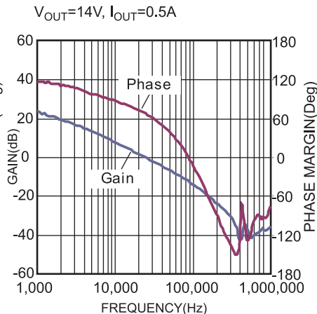
Bode Plot
