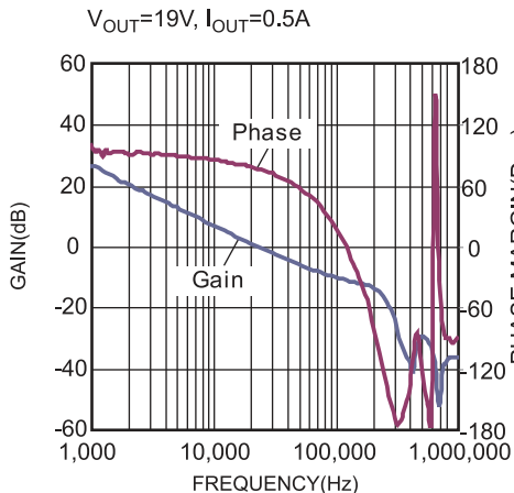
Bode Plot
