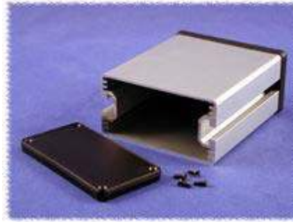
Solid ABS Plastic Bezel Version (Open View)
