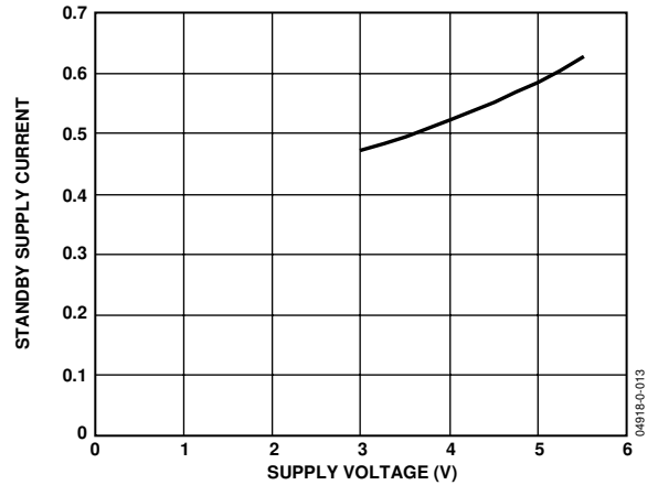
Figure 13. Standby Supply Current vs. Supply Voltage
