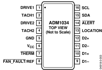
Figure 3. Pin Configuration
