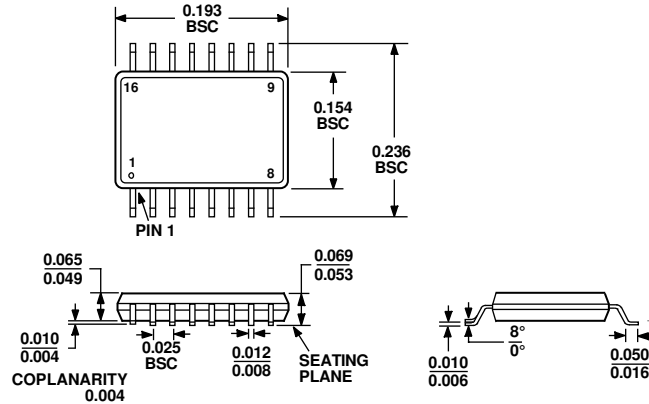
COMPLIANT TO JEDEC STANDARDS MO-137AB Figure 45. 16-Lead Shrink Small Outline Package [QSOP] (RQ-16) Dimensions shown in inches
